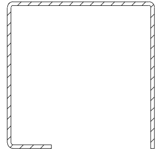
Door Z Sash 105.5mm White Profile Art. No. 546625 Laminated Profile Art. No. 576625
